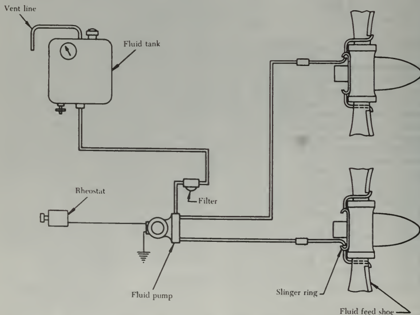
FIGURE 7-25. Typical propeller fluid anti-icing system.
